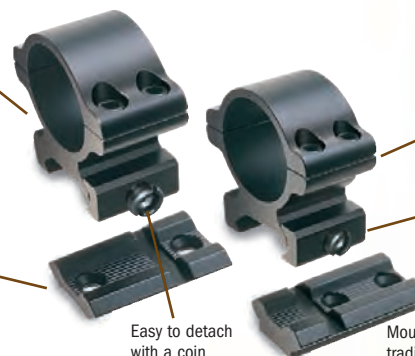
Aluminum Alloy One-Piece Bases
